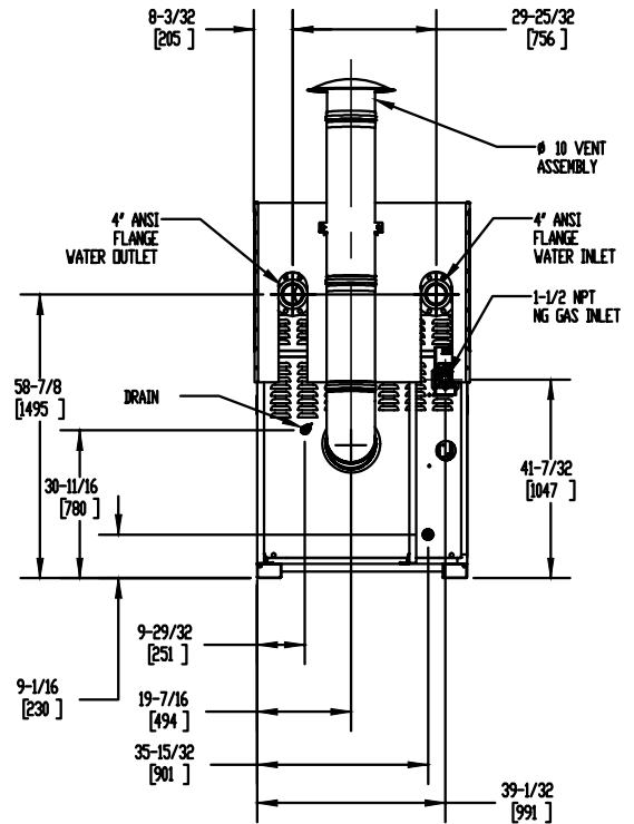
BACK VIEW
