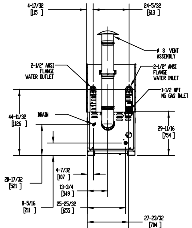
BACK VIEW
